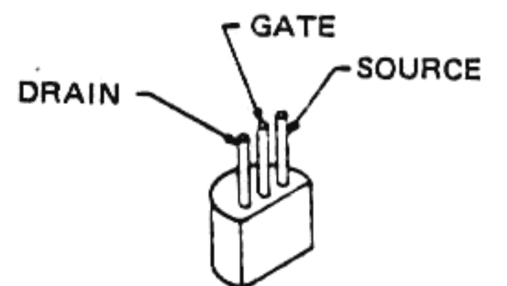
2SK107-3
