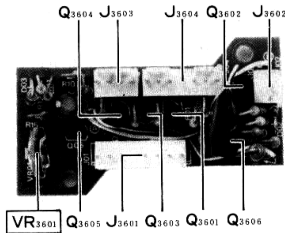
MONITOR UNIT
