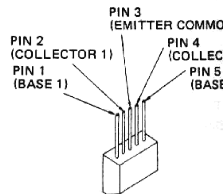
2SC1583G
